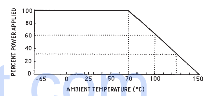
POWER DERATING
