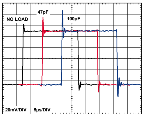
Figure 35. Small Signal Pulse Response for Various Capacitive Loads, V_S = \pm 15\text{ V} , V_{REF} = 0\text{ V}
