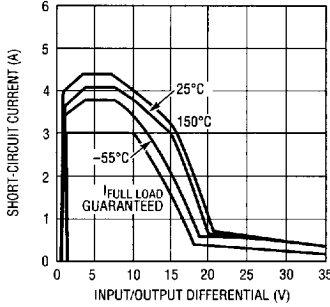
LT1085 Short-Circuit Current
