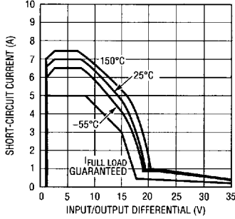
LT1084 Short Circuit Current
