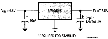
5V, 7.5A Regulator
