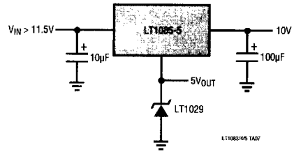
Regulator with Reference
