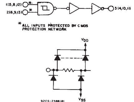
Fig. 1 – Logic diagram—1 of 4 Schmitt triggers.
