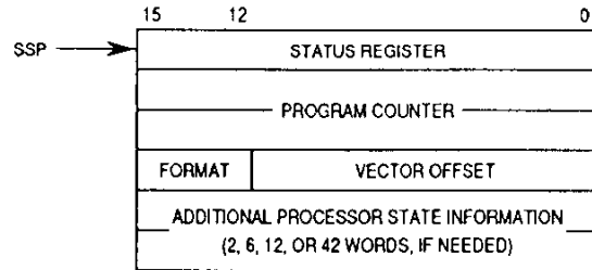
Figure 2-1. General Exception Stack Frame
