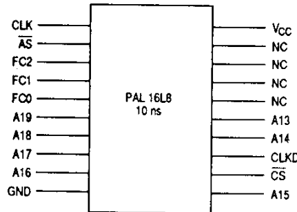
Figure 9-2. Chip Select Generation PAL
