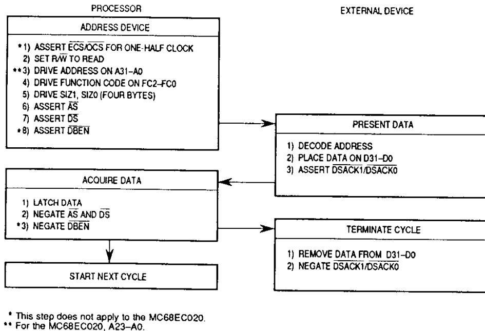
Figure 5-19. Long-Word Read Cycle Flowchart
