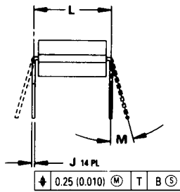
J SUFFIX CERAMIC CASE 632-08
