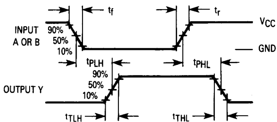
Figure 1. Switching Waveforms
