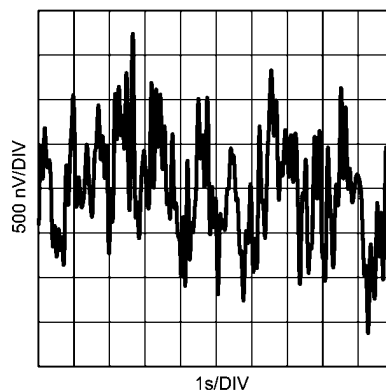
0.1Hz to 10Hz Noise (Core op-amp)
