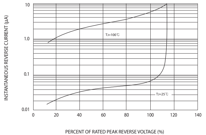
FIG.4-TYPICAL REVERSE CHARACTERISTICS
