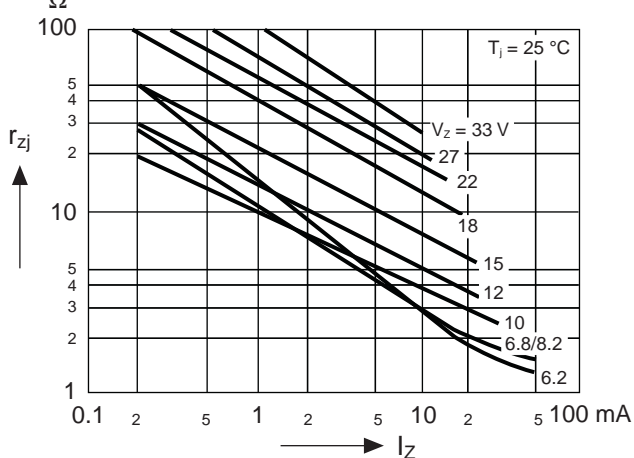
Dynamic resistance versus Zener current
