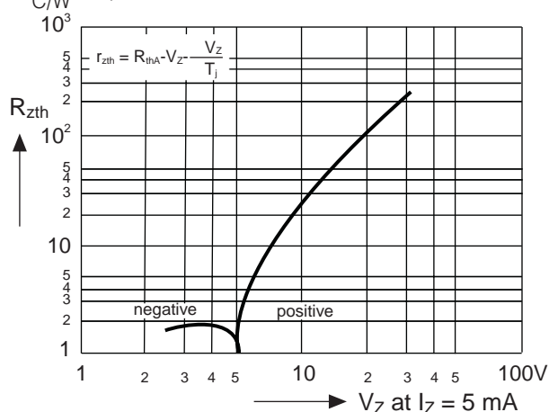
Thermal differential resistance versus Zener voltage
