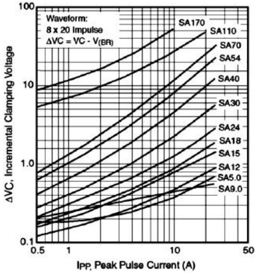
Fig. 7 – Incremental Clamping Voltage Curve Unidirectional
