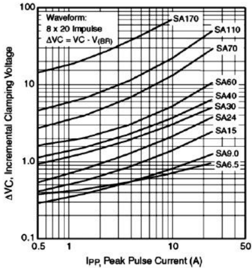
Fig. 9 – Incremental Clamping Voltage Curve Bidirectional
