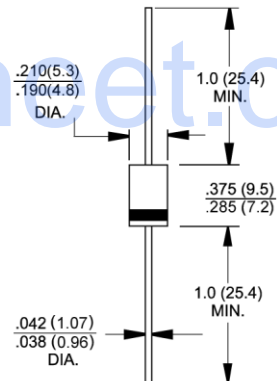
DO-201AE
