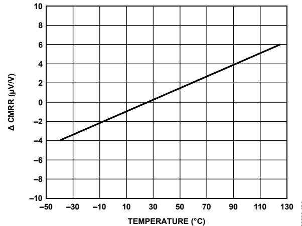
Figure 20. Change in CMRR vs. Temperature, G = 1
