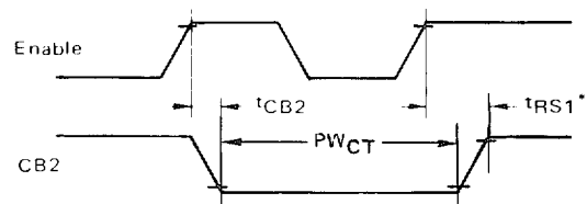
FIGURE 11 — CB2 DELAY TIME (Write Mode; CRB-5=CRB-3=1, CRB-4=0)
