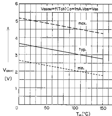
Gate Threshold Voltage vs. T_{ch}
