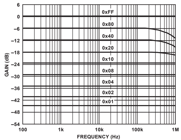
Figure 19. AD5242 10 kΩ Gain vs. Frequency vs. Code
